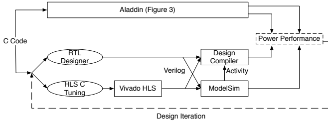
Figure 6: Validation Flow.
